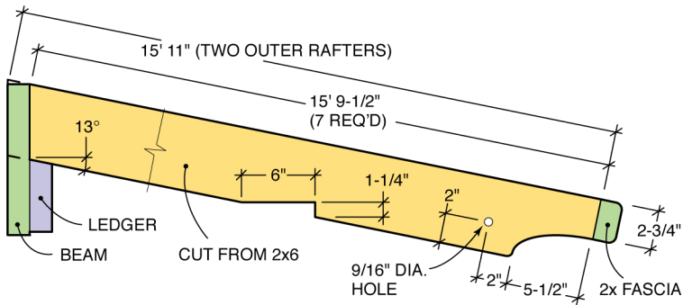
Fig. D Rafter Detail
