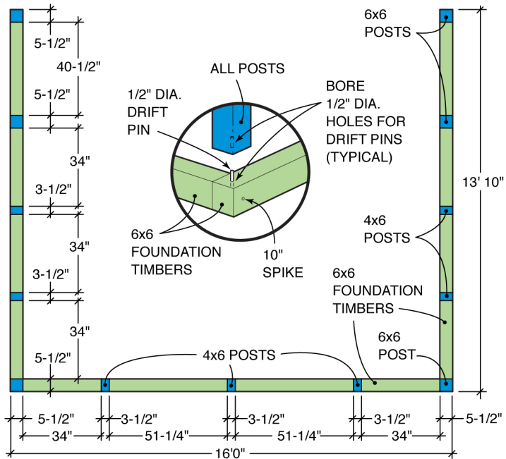
Fig. A Foundation & Post Layout
