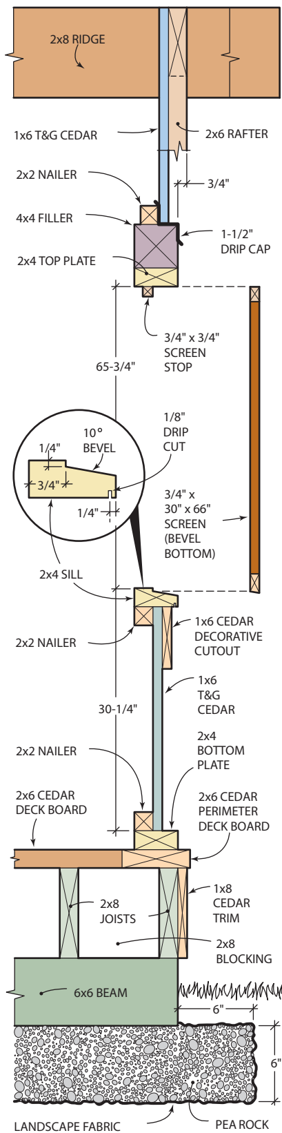
GABLE WALL SECTION VIEW
