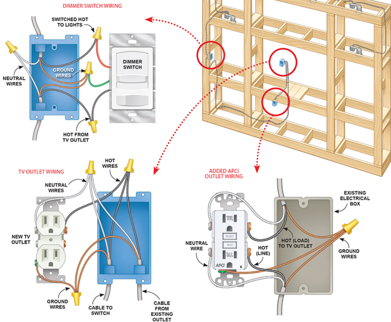
Figure B Electrical diagrams
