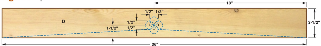
Figure D Apron detail
