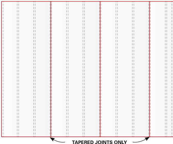
Figure B Drywall parallel to joists
