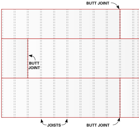
Figure A Drywall perpendicular to joists
