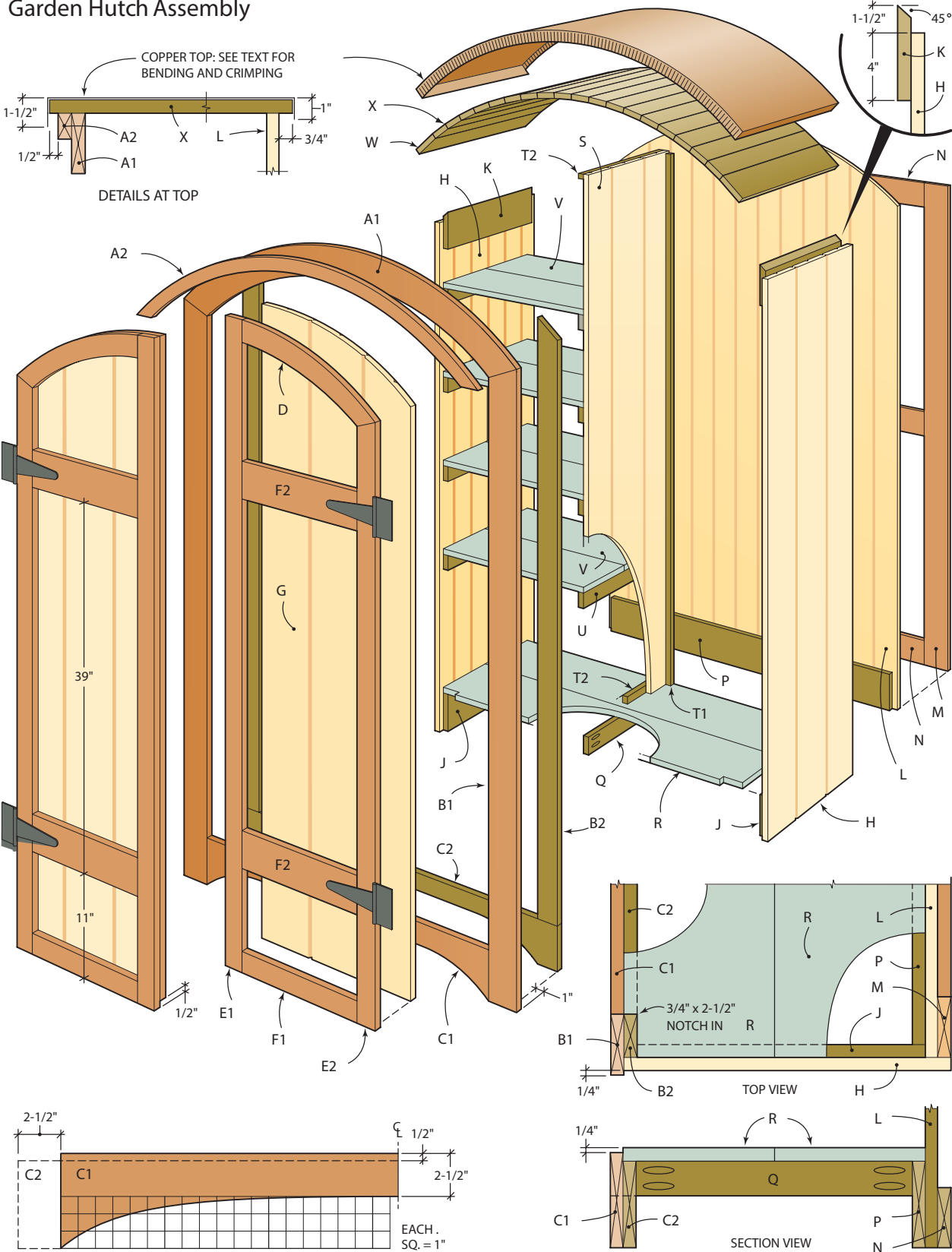
Figure A Garden Hutch Assembly
