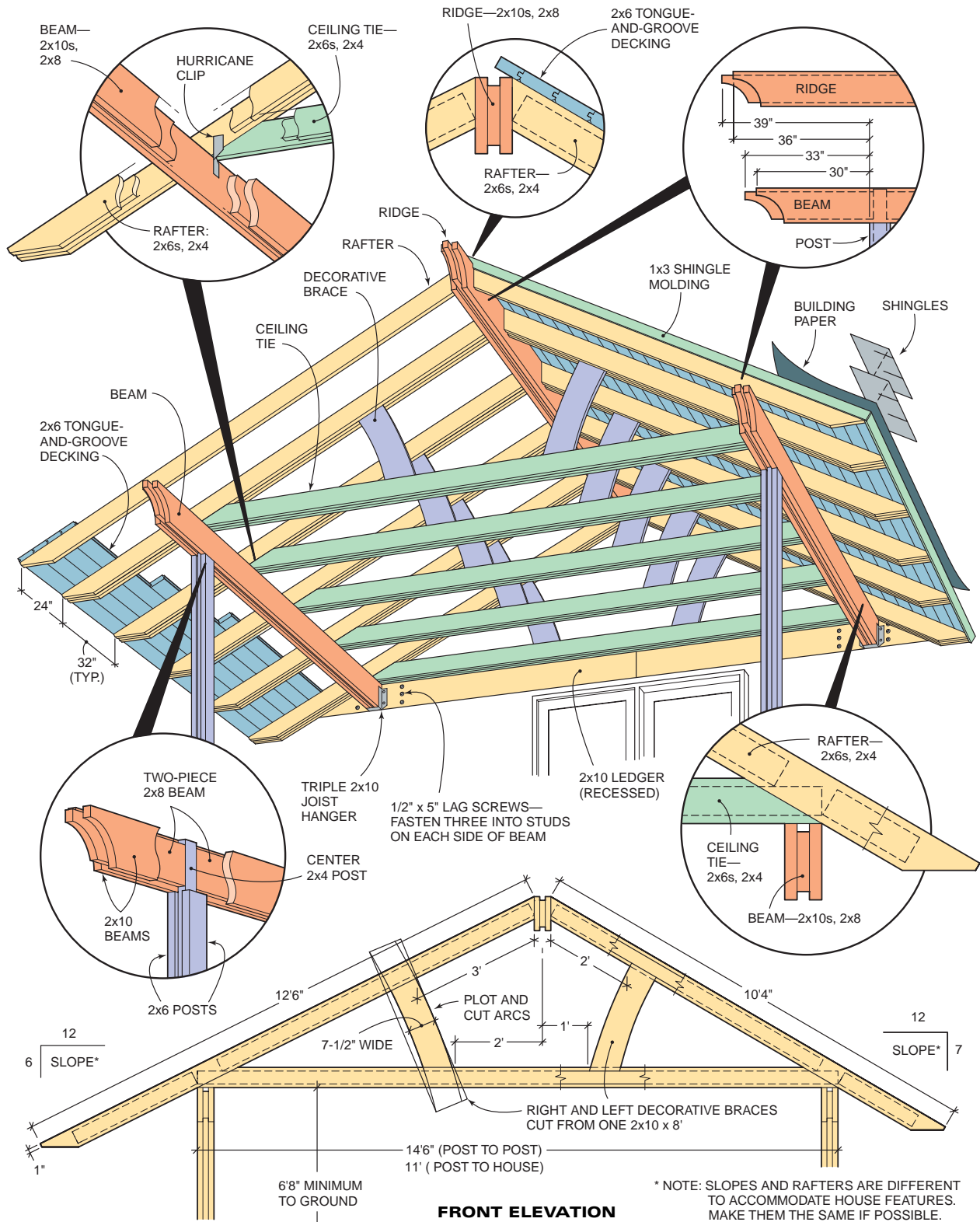
FIG. A ROOF ASSEMBLY
