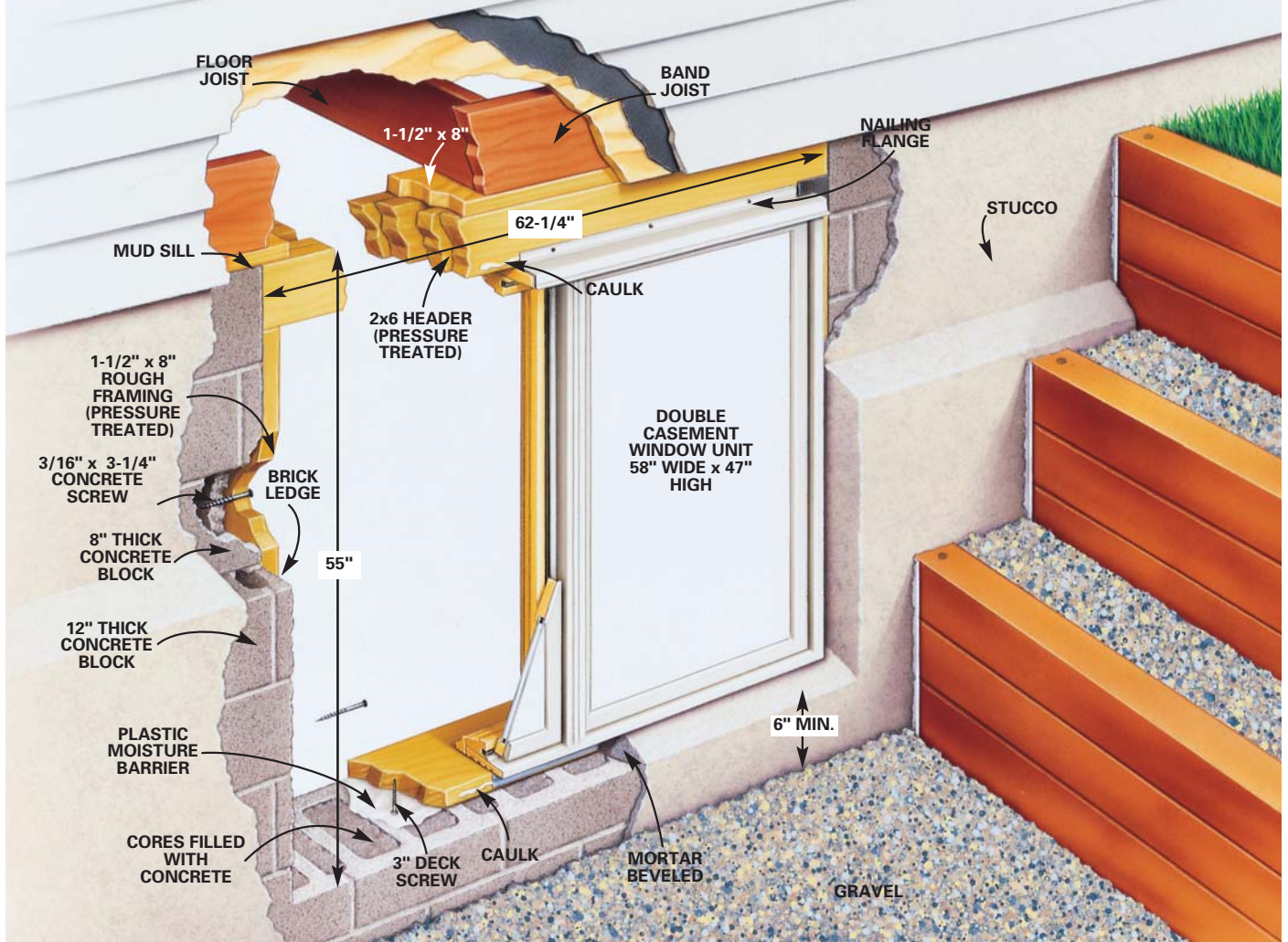
FIG. A WINDOW FRAMING DETAILS
