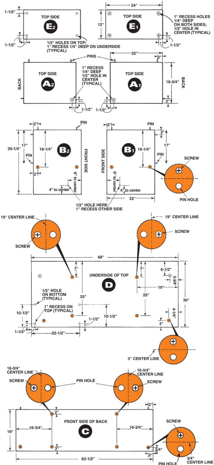
Fig. B Fastener Location Guide
