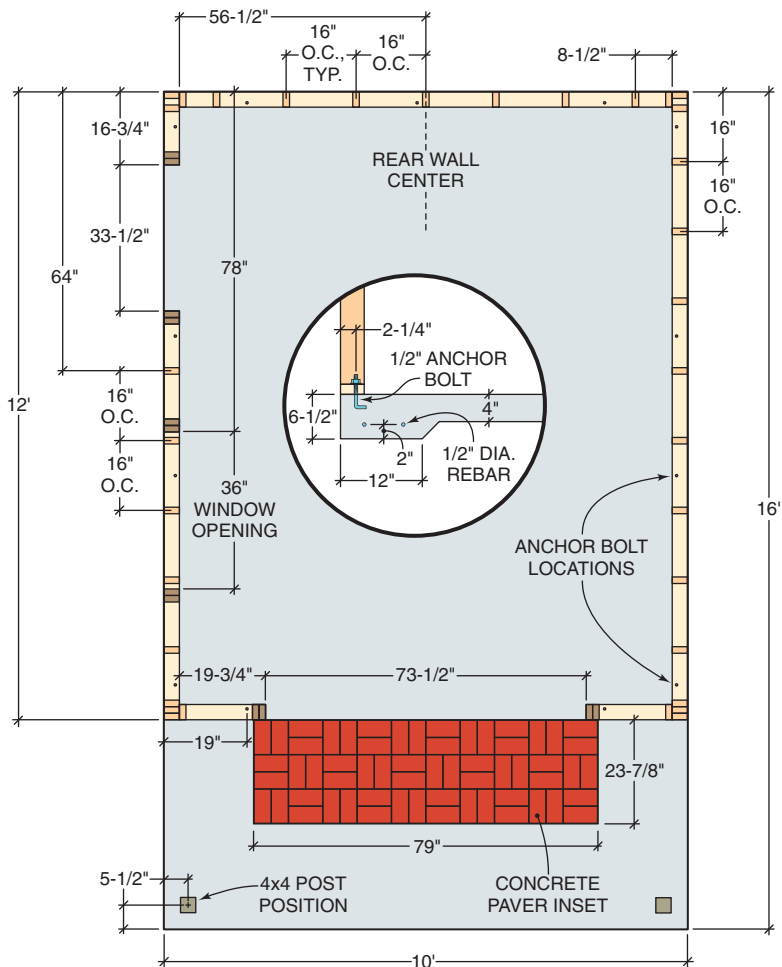
Figure A Slab and stud detail
